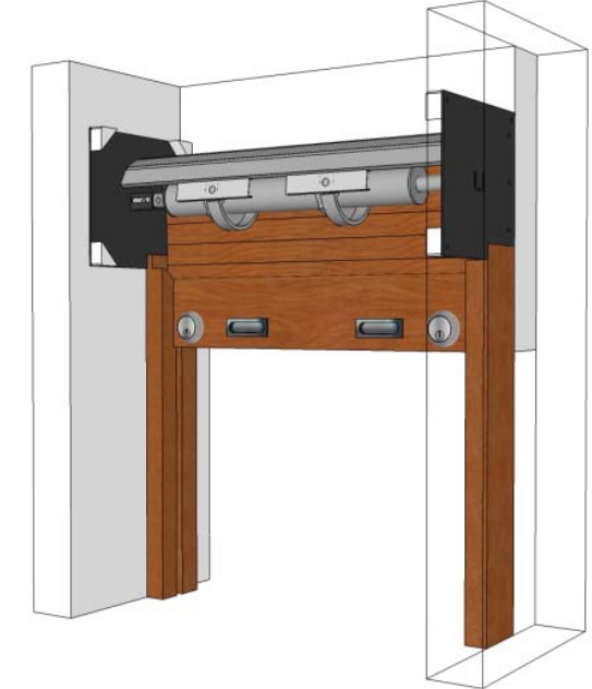
Between Wall Mount on Face of Lintel
