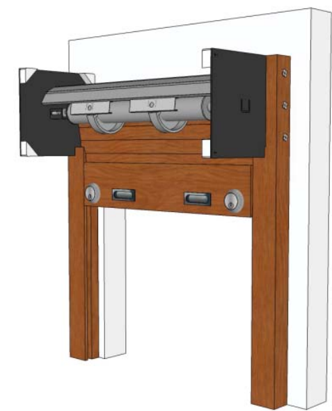
Outside Mount
